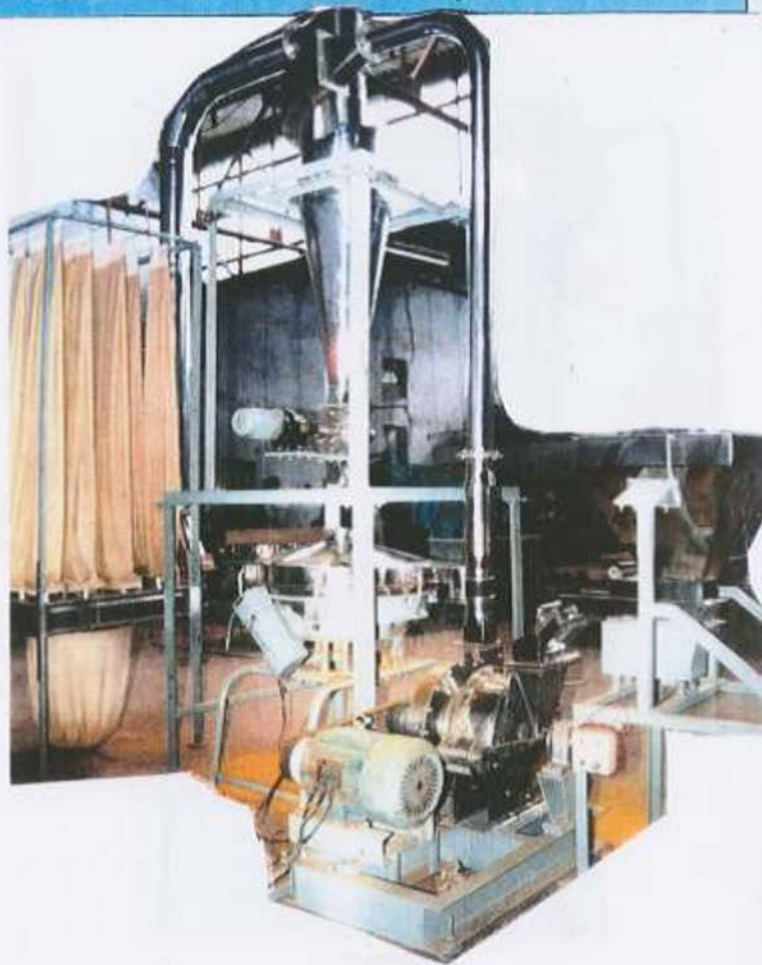
"FINEX" AIR SWEEP MILL (SCREENLESS)
